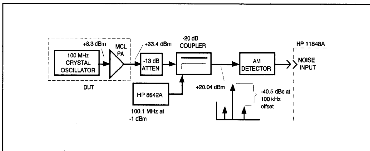
Figure 3-20. Source Without AM Measurement Setup
