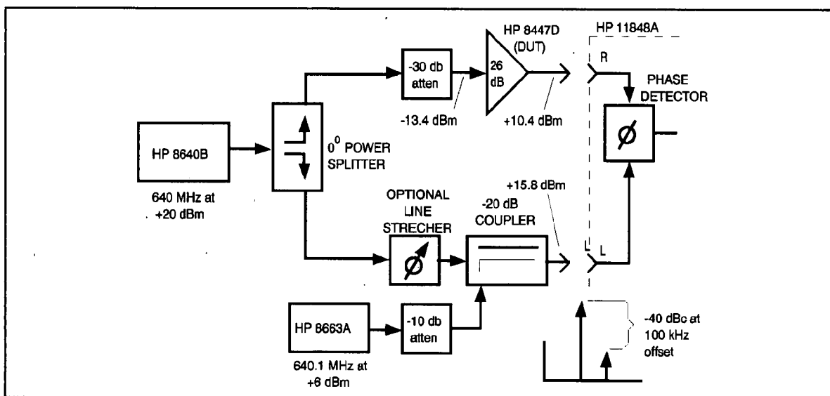
Figure 2-22. Dynamic Noise Figure Measurement Setup
