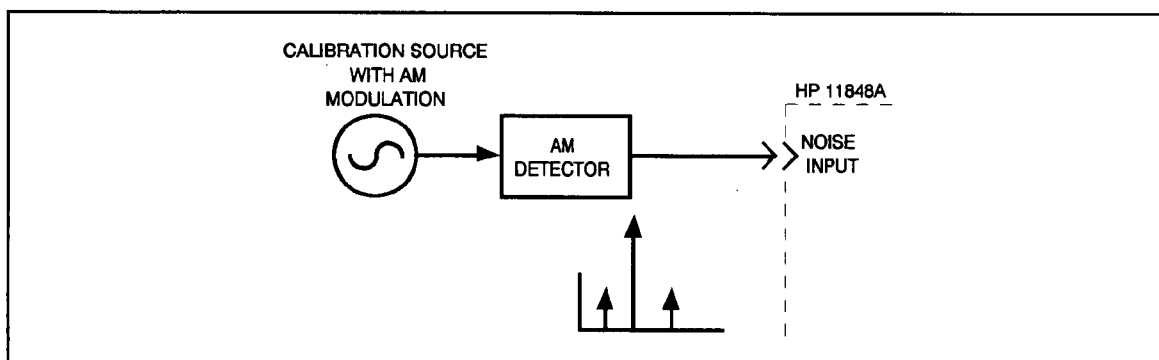
Figure 3-14. Measuring the Calibration Constant
