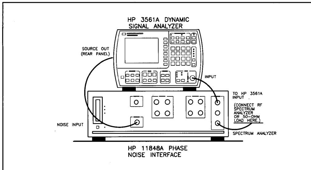
Figure 29. Third Option 2 Calibration Setup
