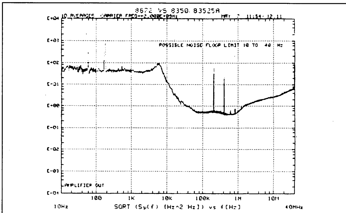
Figure 2-4. S_{\phi}(f) : Spectral Density of Phase Fluctuation
