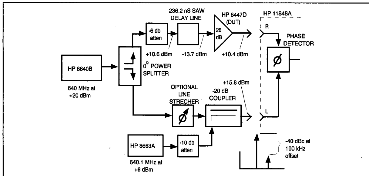
Figure 2-24. Time Delay Measurement Setup
